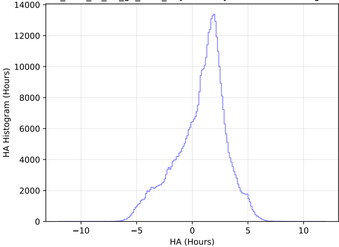
too_elab_r8_d3_gz_v3.4_10yrs All sky z band: HA Histogram
