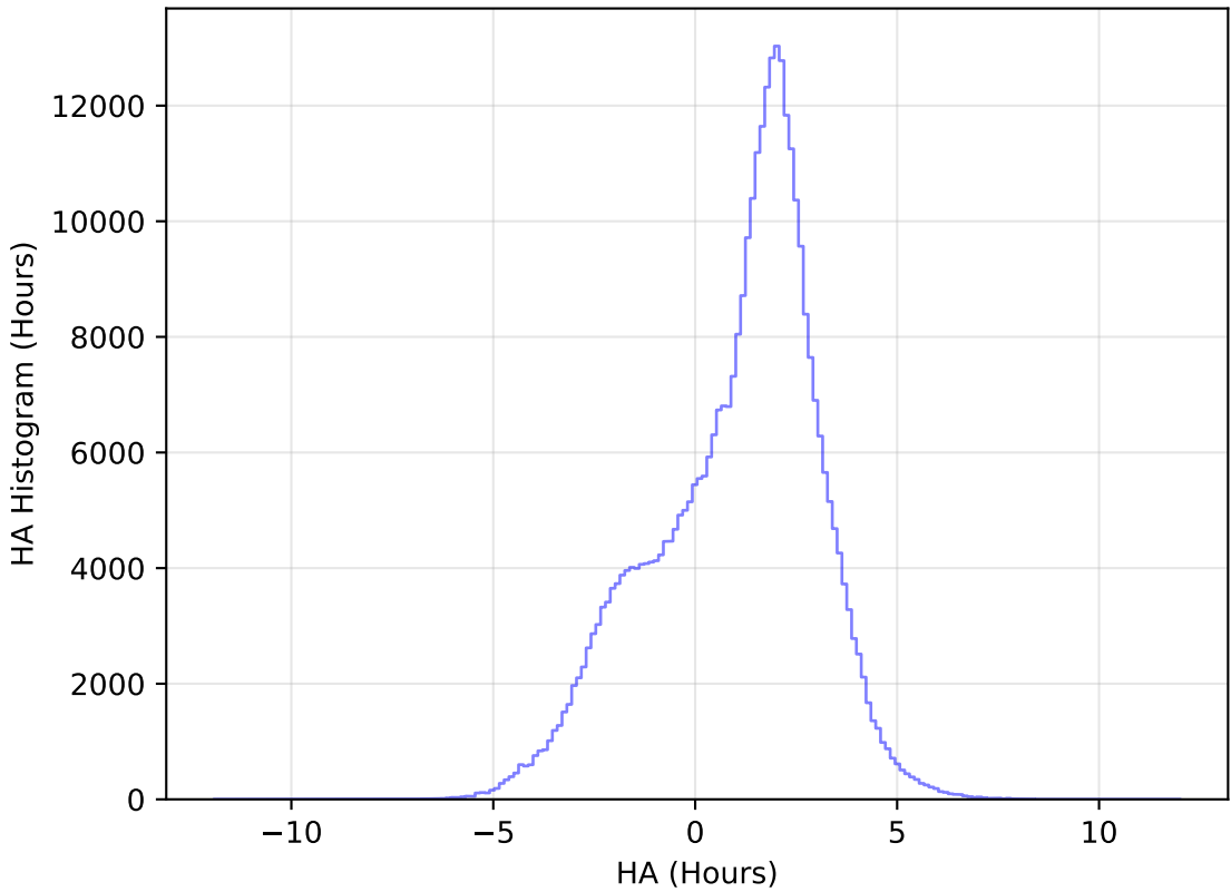
too_elab_r8_d3_gz_v3.4_10yrs All sky y band: HA Histogram
