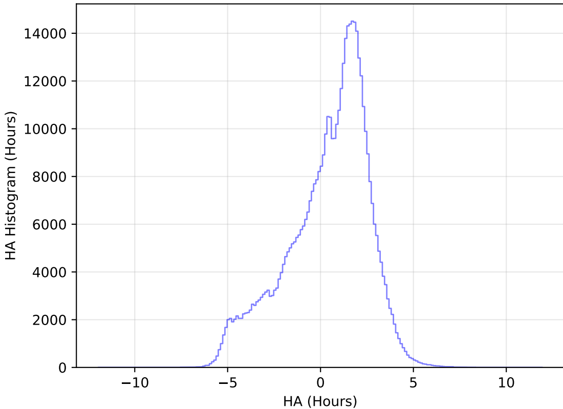
too_elab_r8_d3_gz_v3.4_10yrs All sky r band: HA Histogram
