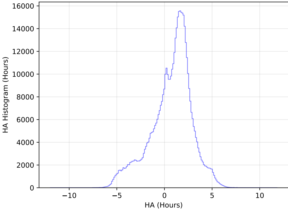
too_elab_r8_d3_gz_v3.4_10yrs All sky i band: HA Histogram
