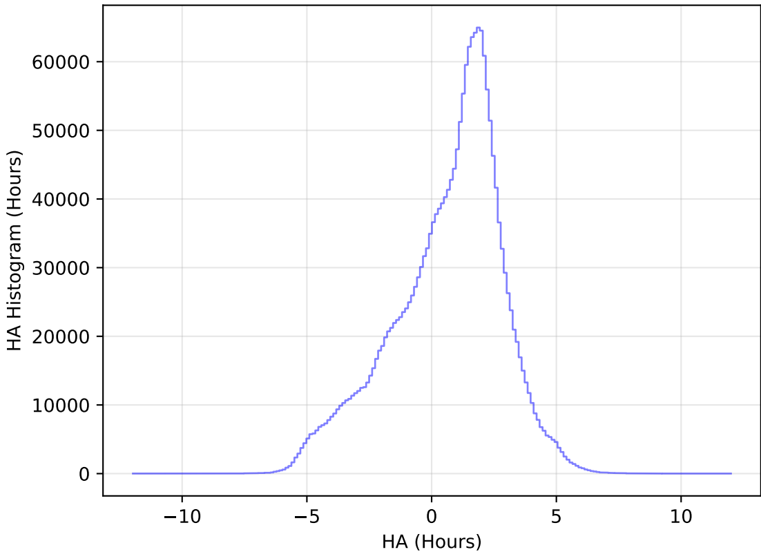
too_elab_r8_d3_gz_v3.4_10yrs All sky all bands: HA Histogram
