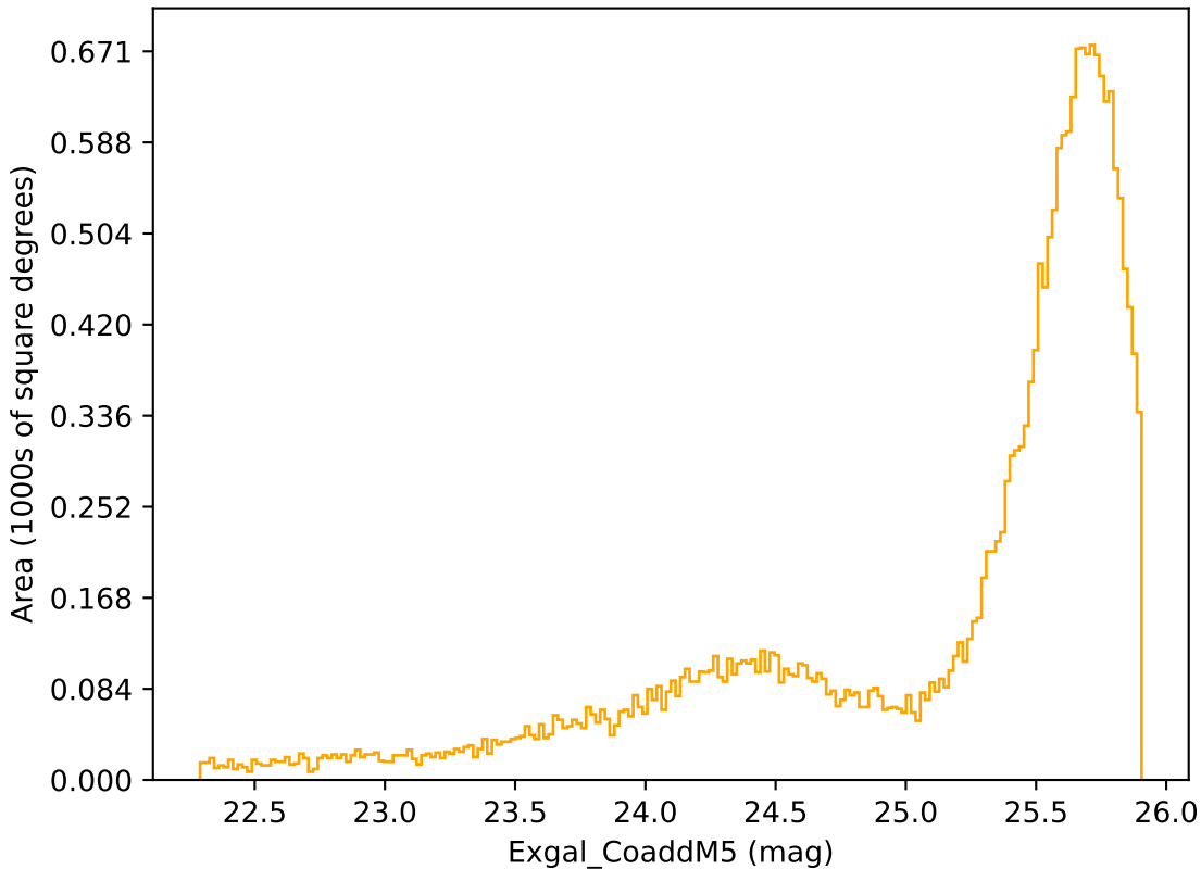
too_elab_r8_d3_gz_v3.4_10yrs Yr 1 r band: Exgal_CoaddM5
