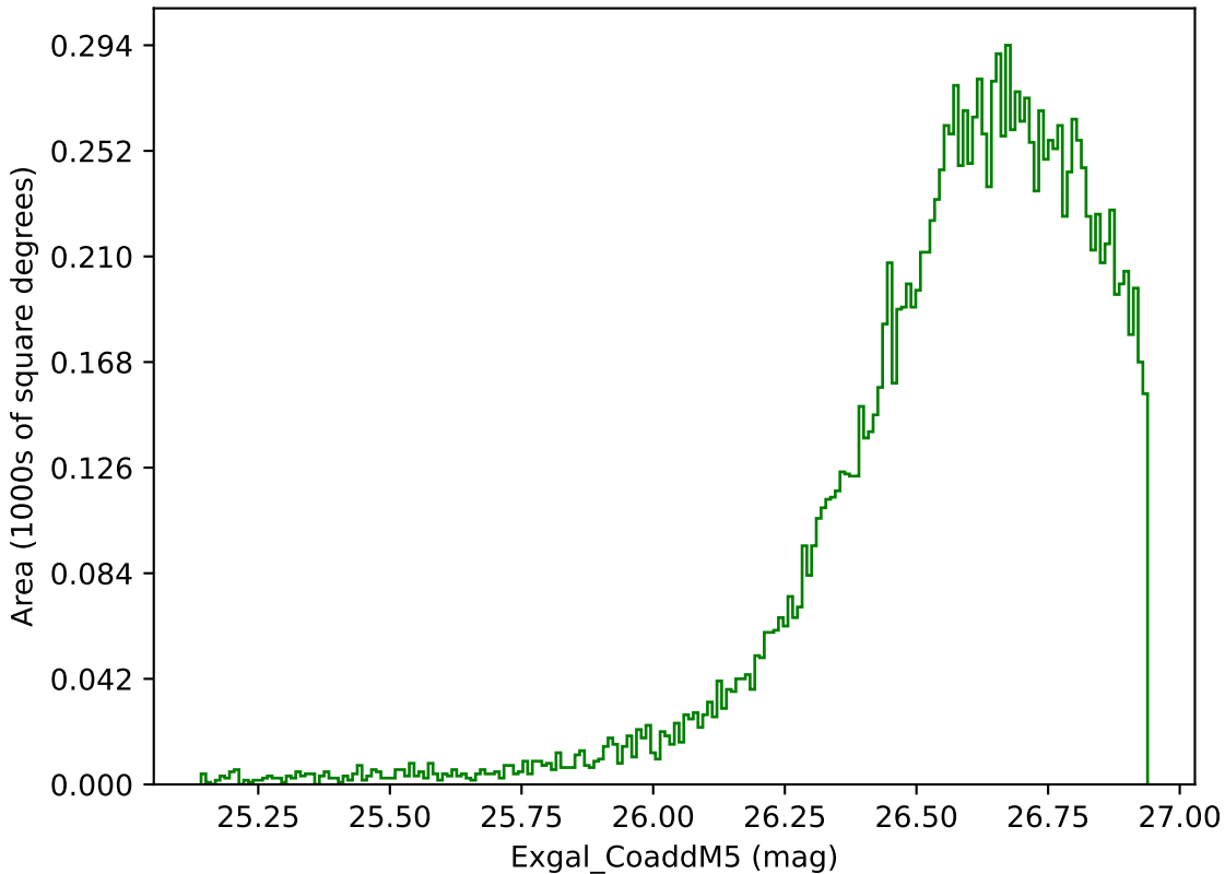
too_elab_r8_d3_gz_v3.4_10yrs WFD g band: Exgal_CoaddM5
