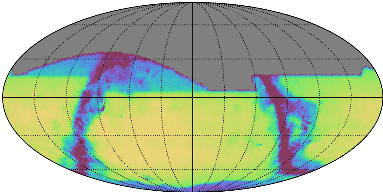
too_elab_r8_d3_gz_v3.4_10yrs All sky z band: Exgal_CoaddM5
