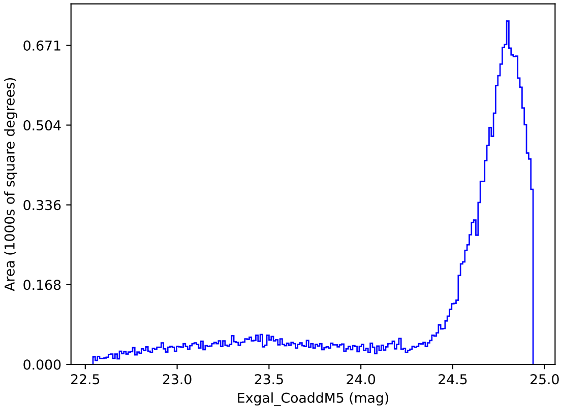
too_elab_r8_d3_gz_v3.4_10yrs All sky y band: Exgal_CoaddM5
