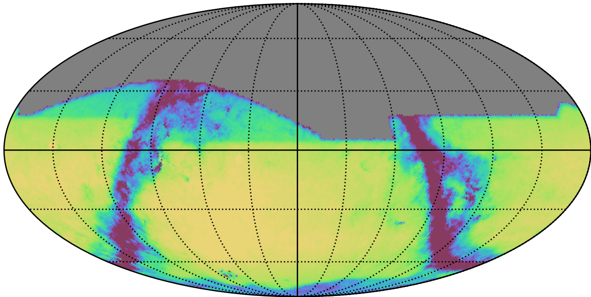
too_elab_r8_d3_gz_v3.4_10yrs All sky r band: Exgal_CoaddM5
