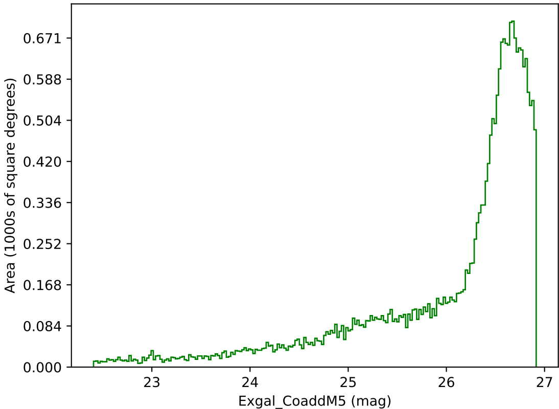
too_elab_r8_d3_gz_v3.4_10yrs All sky g band: Exgal_CoaddM5
