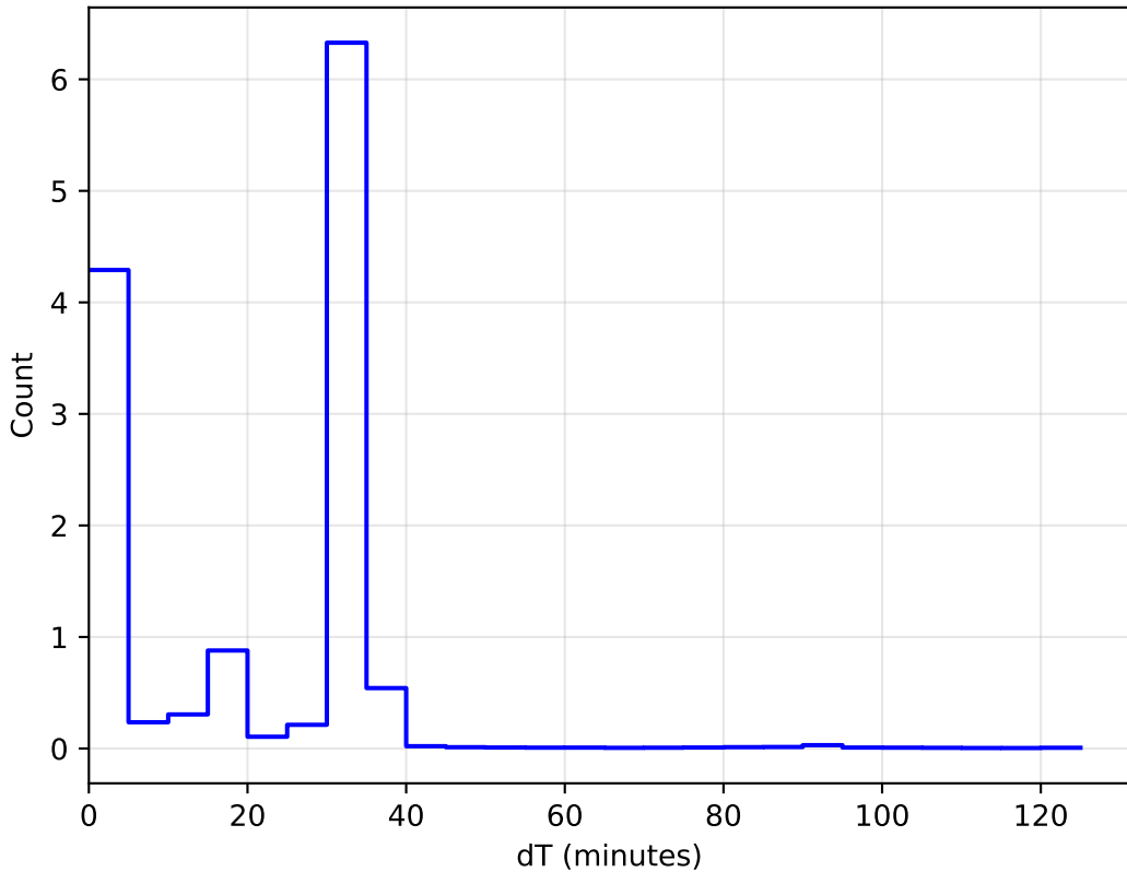
too_elab_r8_d3_gz_v3.4_10yrs All sky: DeltaT Histogram
