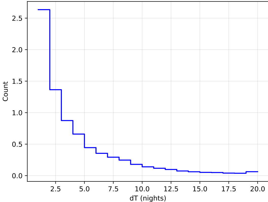
too_elab_r8_d3_gz_v3.4_10yrs WFD all bands: DeltaNight Histogram 1e6
