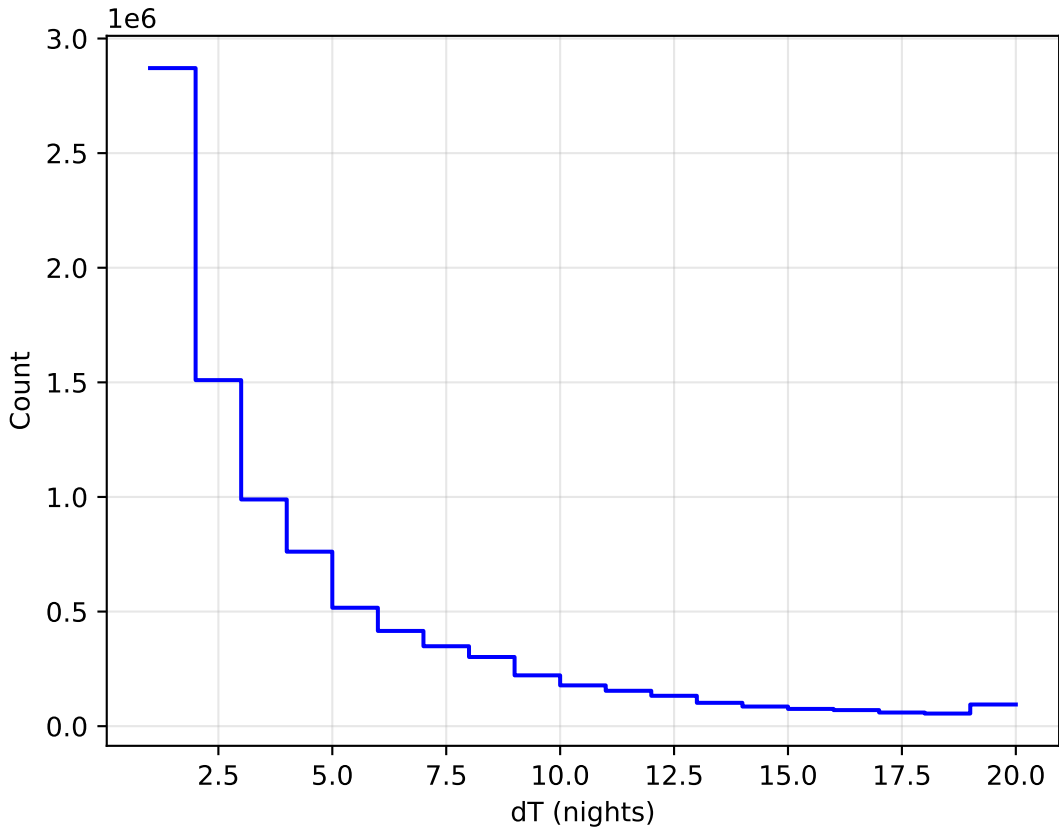
too_elab_r8_d3_gz_v3.4_10yrs All sky all bands: DeltaNight Histogram
