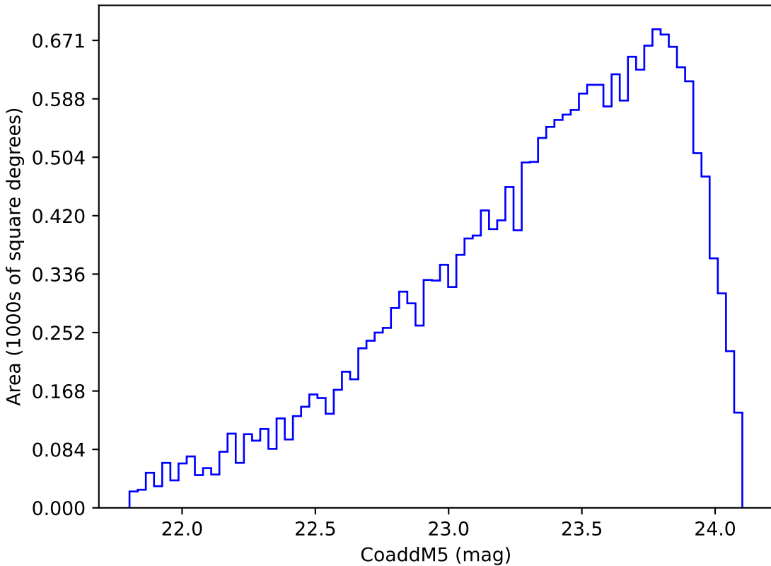
too_elab_r8_d3_gz_v3.4_10yrs Yr 3-4 y band: CoaddM5
