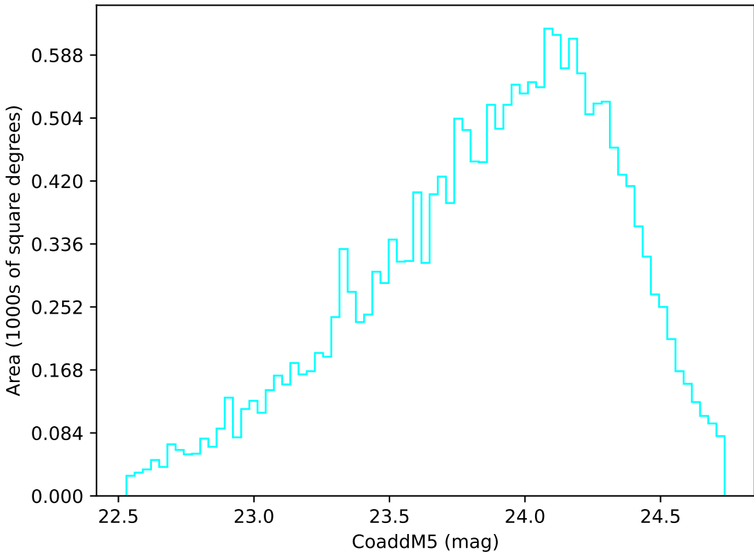
too_elab_r8_d3_gz_v3.4_10yrs Yr 3-4 u band: CoaddM5
