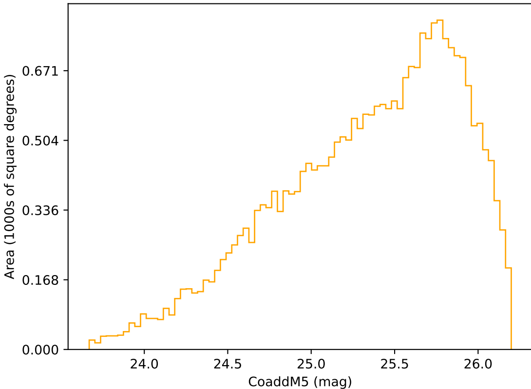
too_elab_r8_d3_gz_v3.4_10yrs Yr 3-4 r band: CoaddM5
