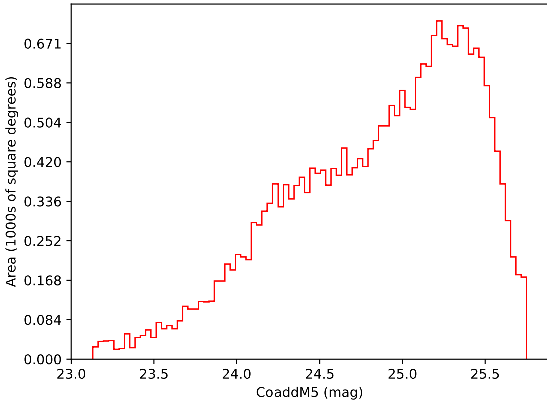
too_elab_r8_d3_gz_v3.4_10yrs Yr 3-4 i band: CoaddM5
