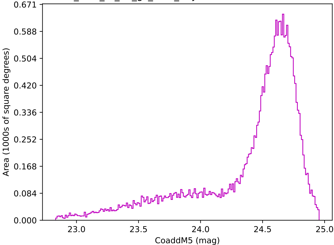
too_elab_r8_d3_gz_v3.4_10yrs Yr 1 z band: CoaddM5
