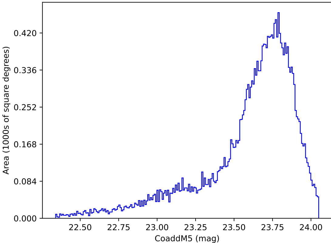
too_elab_r8_d3_gz_v3.4_10yrs Yr 1 y band: CoaddM5
