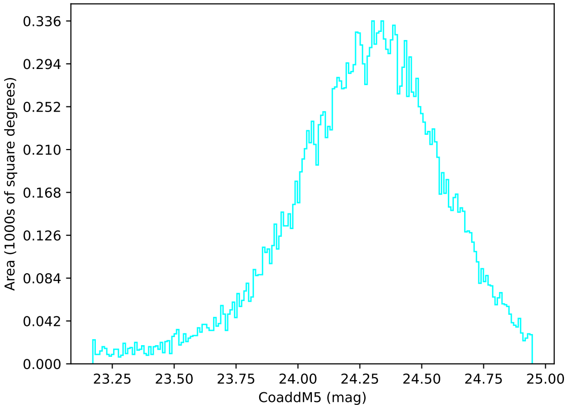
too_elab_r8_d3_gz_v3.4_10yrs Yr 1 u band: CoaddM5
