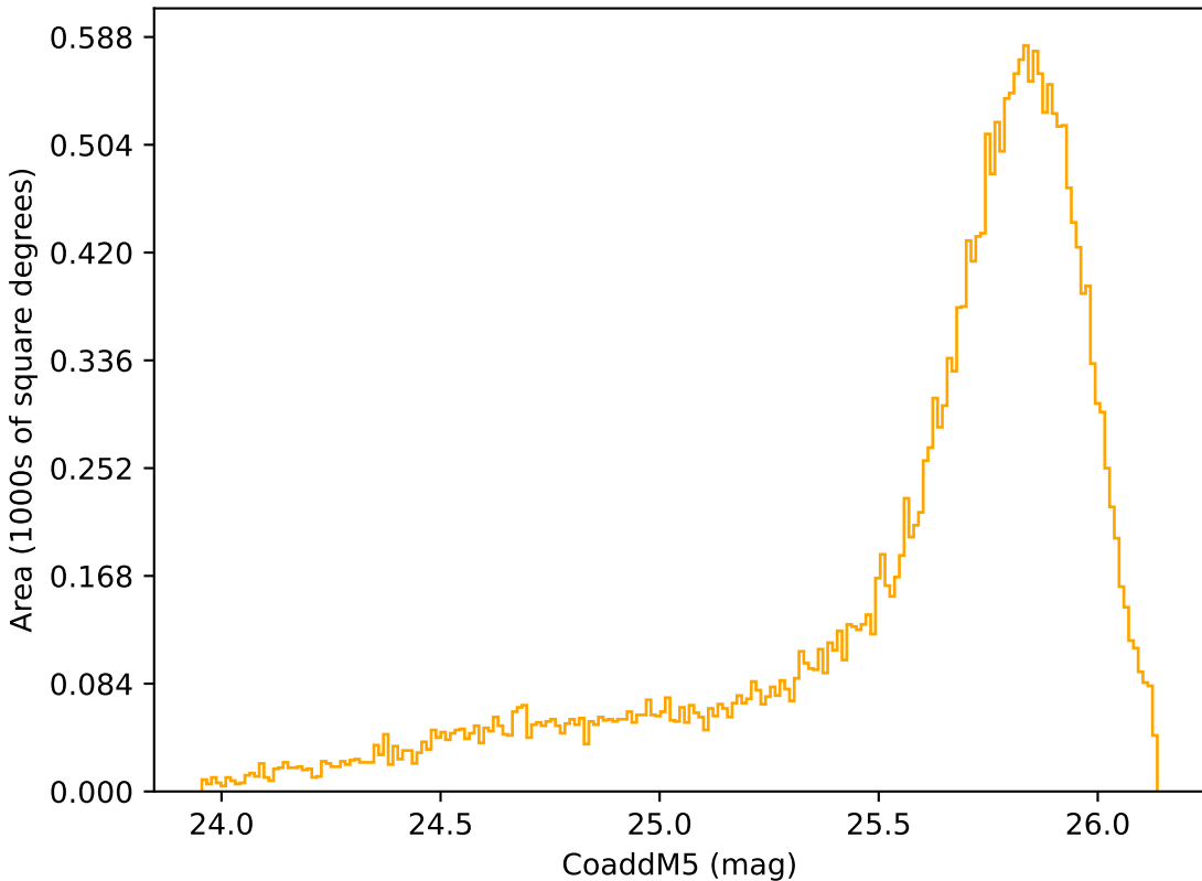
too_elab_r8_d3_gz_v3.4_10yrs Yr 1 r band: CoaddM5
