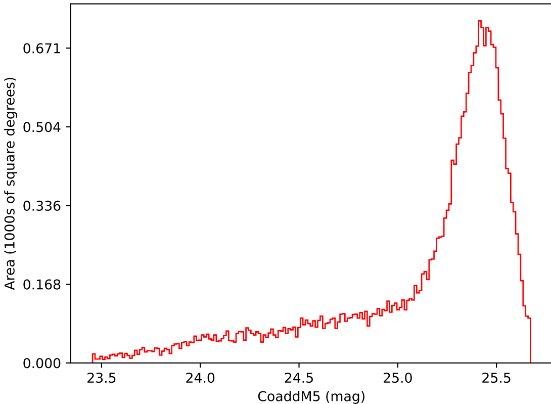
too_elab_r8_d3_gz_v3.4_10yrs Yr 1 i band: CoaddM5
