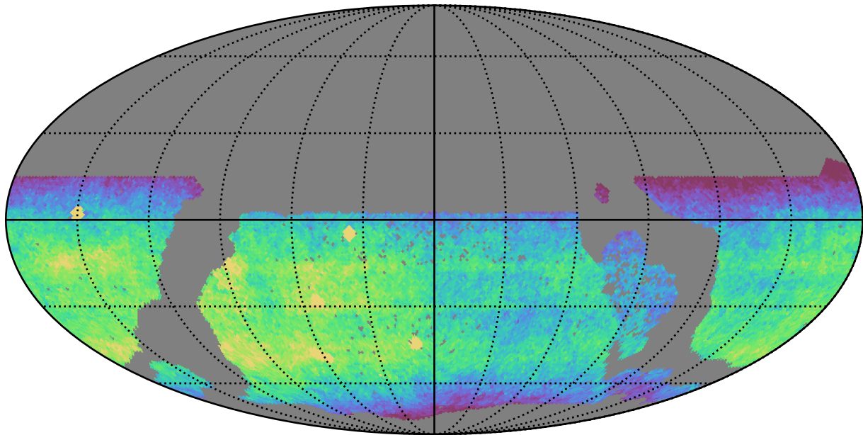
too_elab_r8_d3_gz_v3.4_10yrs WFD z band: CoaddM5
