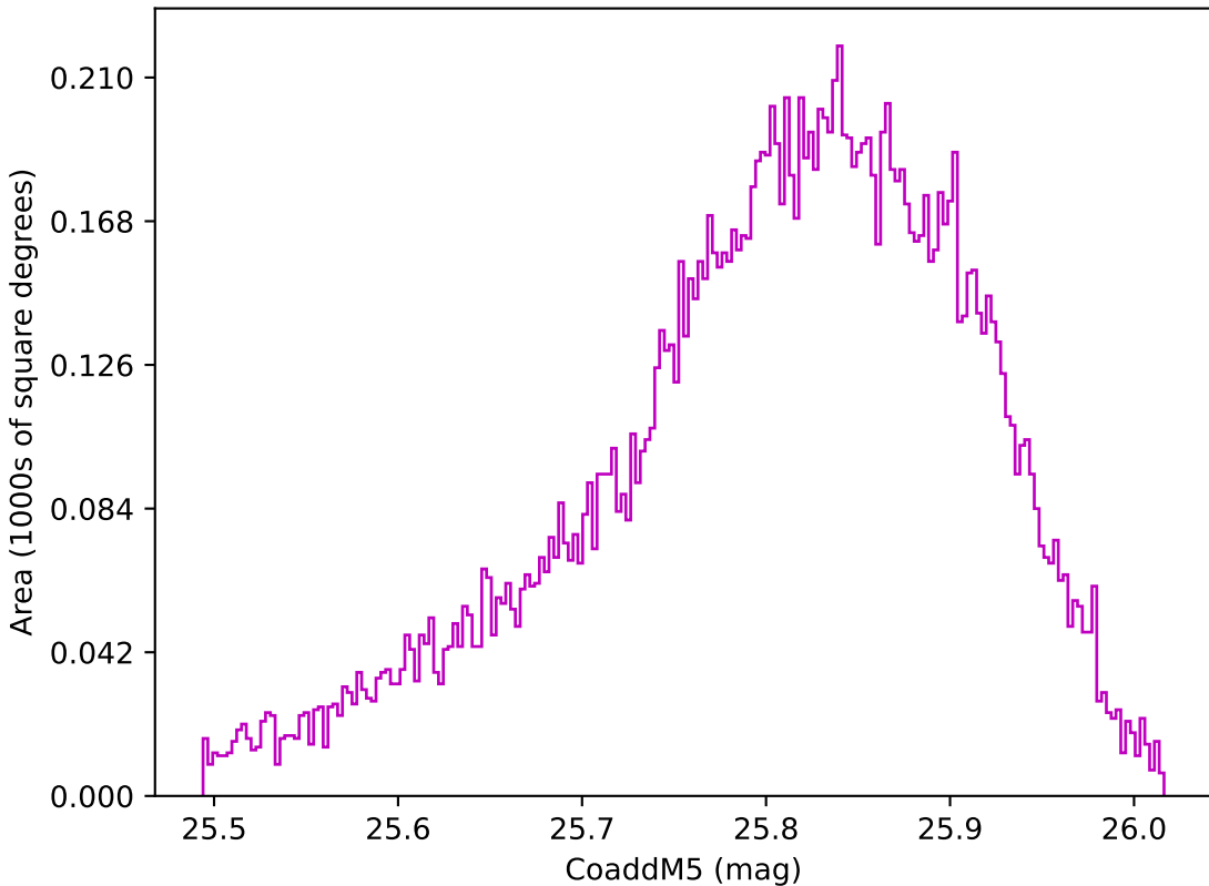
too_elab_r8_d3_gz_v3.4_10yrs WFD z band: CoaddM5
