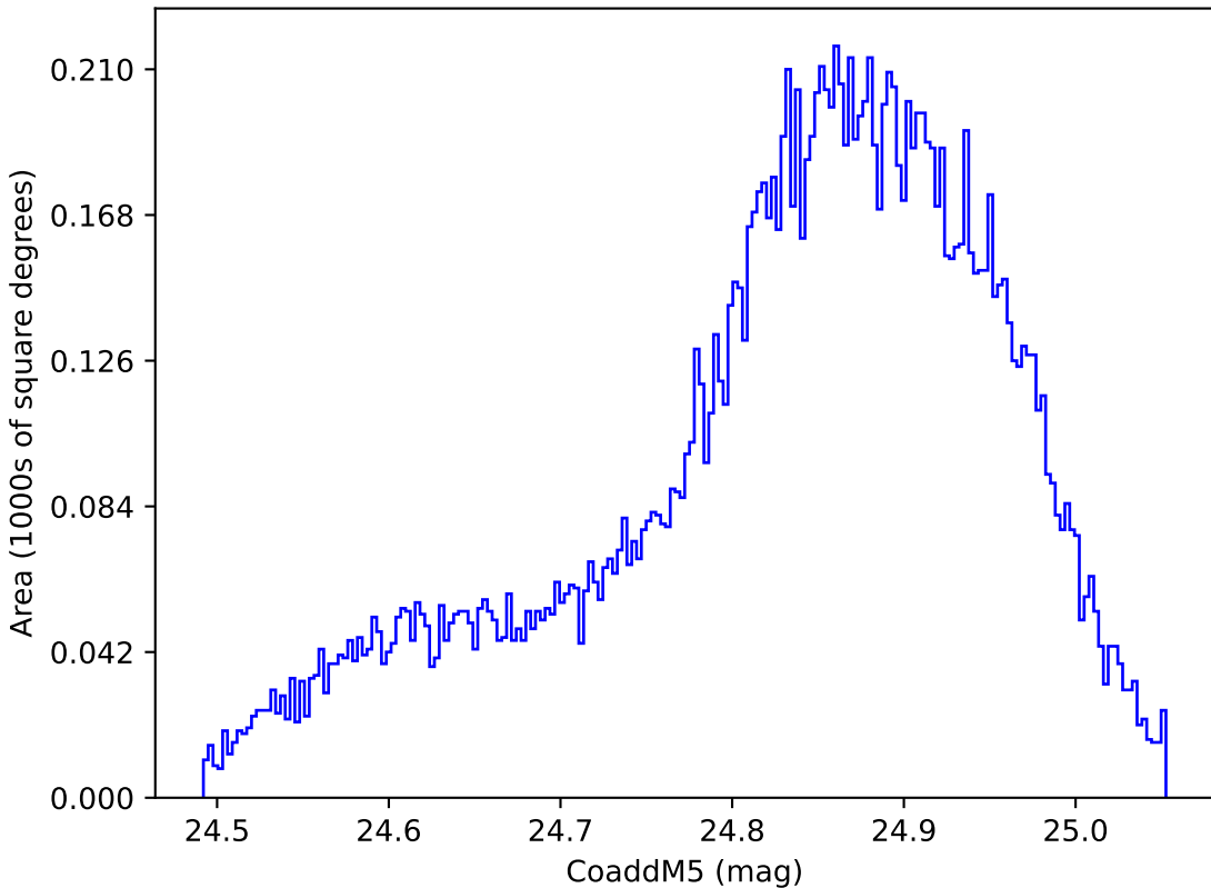
too_elab_r8_d3_gz_v3.4_10yrs WFD y band: CoaddM5
