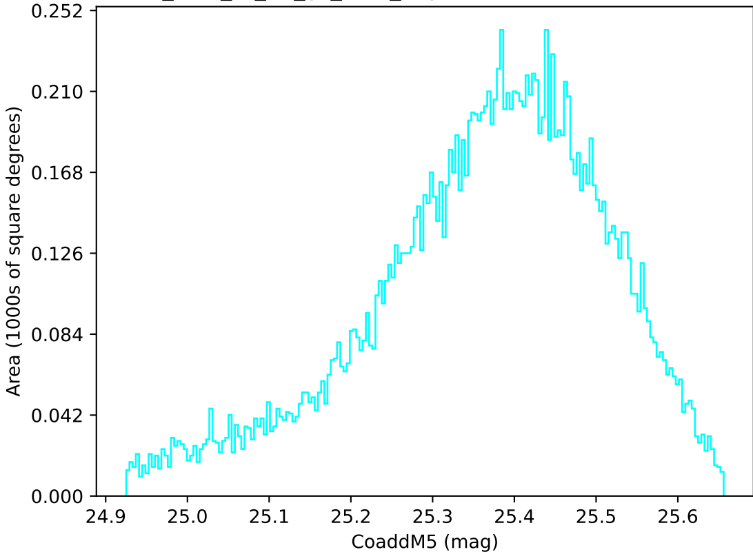
too_elab_r8_d3_gz_v3.4_10yrs WFD u band: CoaddM5
