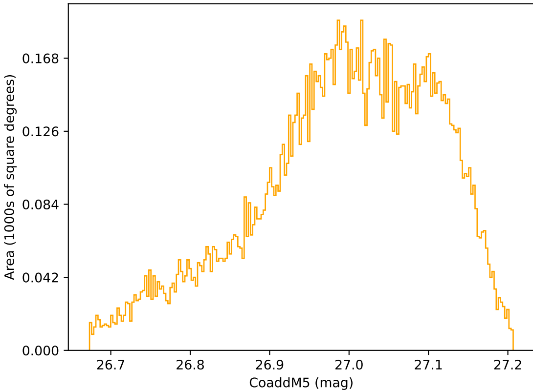
too_elab_r8_d3_gz_v3.4_10yrs WFD r band: CoaddM5
