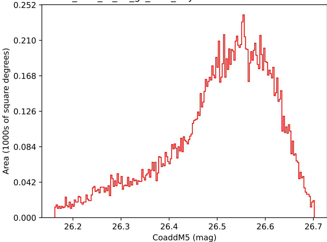
too_elab_r8_d3_gz_v3.4_10yrs WFD i band: CoaddM5
