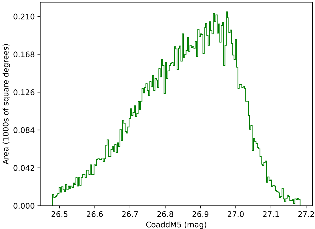
too_elab_r8_d3_gz_v3.4_10yrs WFD g band: CoaddM5
