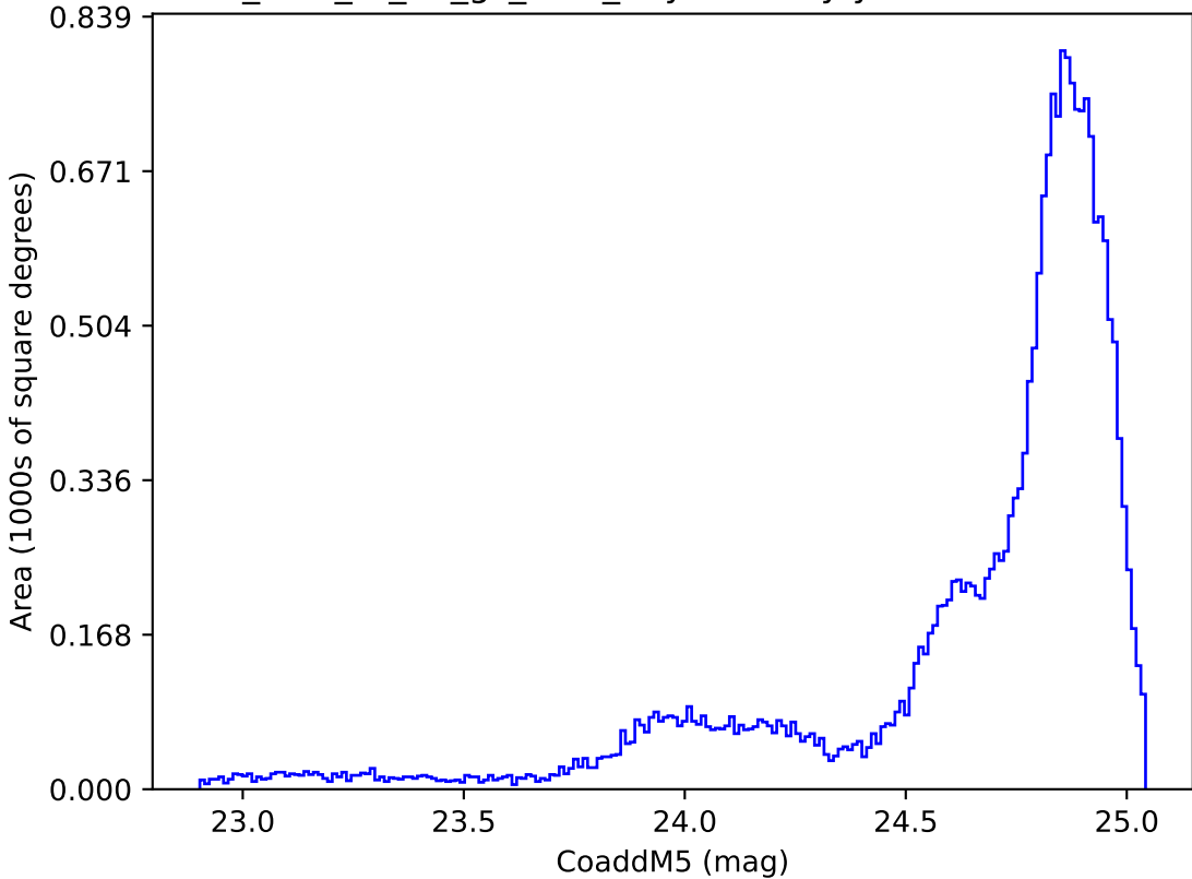
too_elab_r8_d3_gz_v3.4_10yrs All sky y band: CoaddM5
