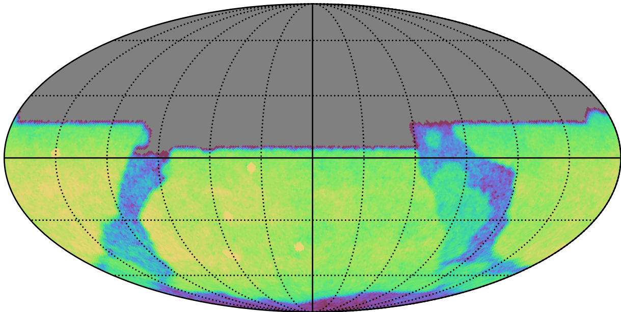
too_elab_r8_d3_gz_v3.4_10yrs All sky u band: CoaddM5
