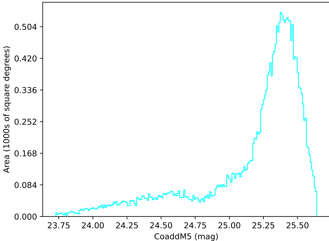
too_elab_r8_d3_gz_v3.4_10yrs All sky u band: CoaddM5
