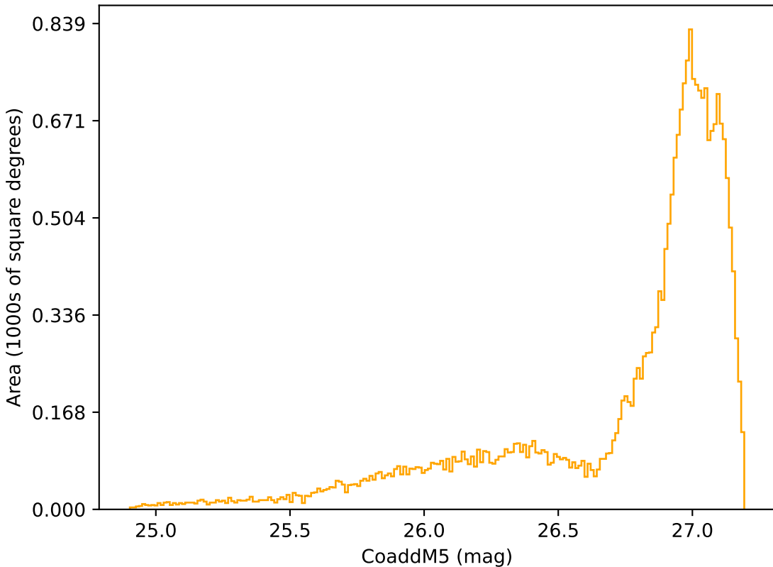
too_elab_r8_d3_gz_v3.4_10yrs All sky r band: CoaddM5
