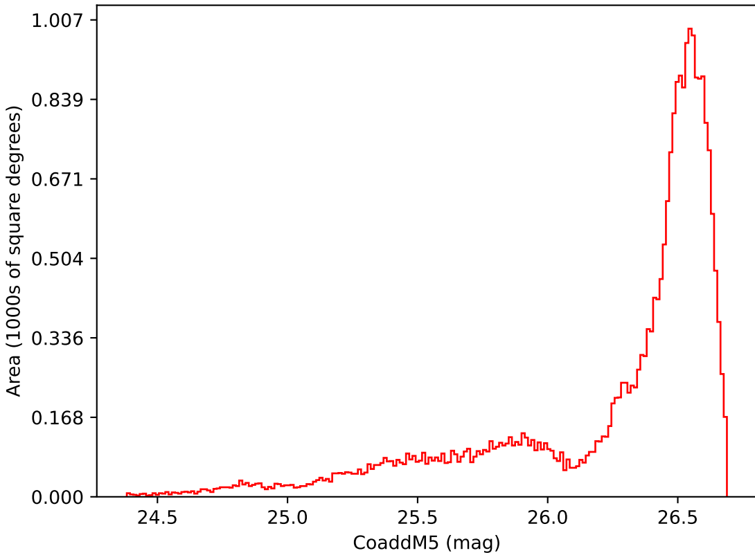
too_elab_r8_d3_gz_v3.4_10yrs All sky i band: CoaddM5
