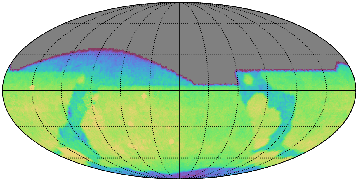
too_elab_r8_d3_gz_v3.4_10yrs All sky g band: CoaddM5
