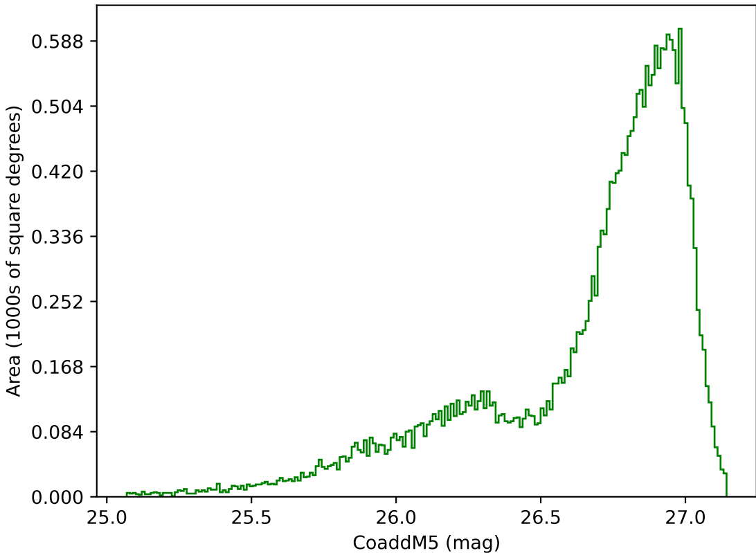
too_elab_r8_d3_gz_v3.4_10yrs All sky g band: CoaddM5
