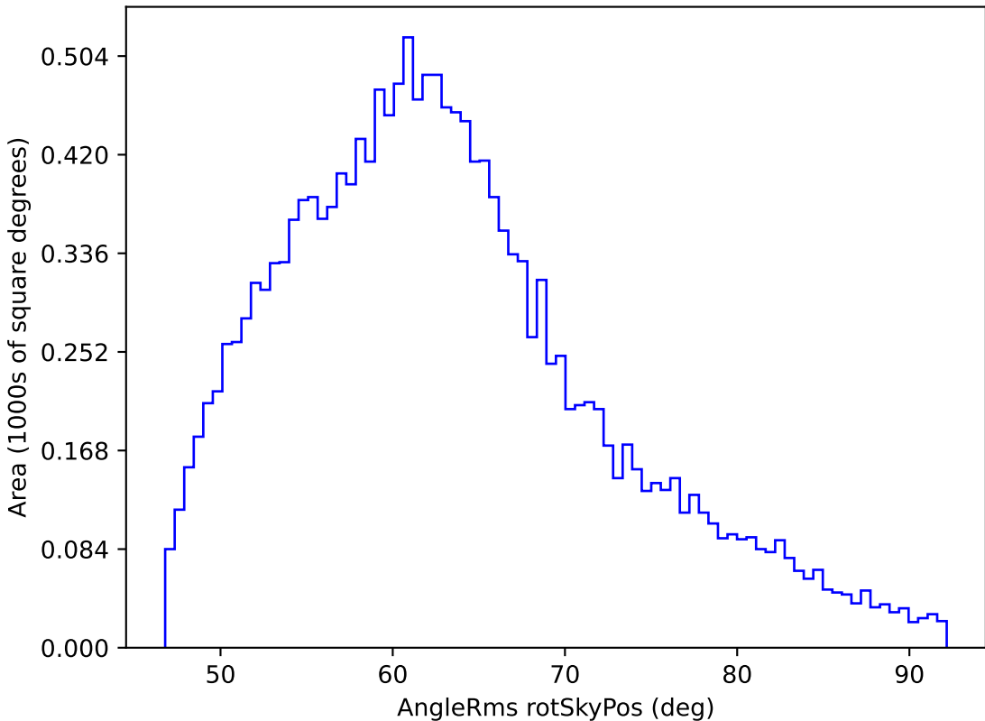
too_elab_r8_d3_gz_v3.4_10yrs WFD y band: AngleRms rotSkyPos
