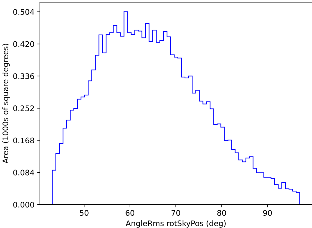
too_elab_r8_d3_gz_v3.4_10yrs WFD u band: AngleRms rotSkyPos
