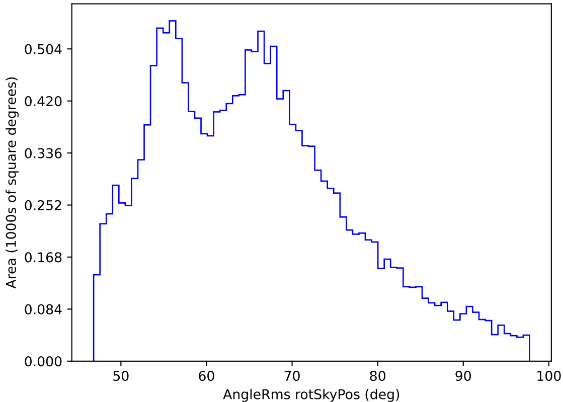
too_elab_r8_d3_gz_v3.4_10yrs WFD r band: AngleRms rotSkyPos
