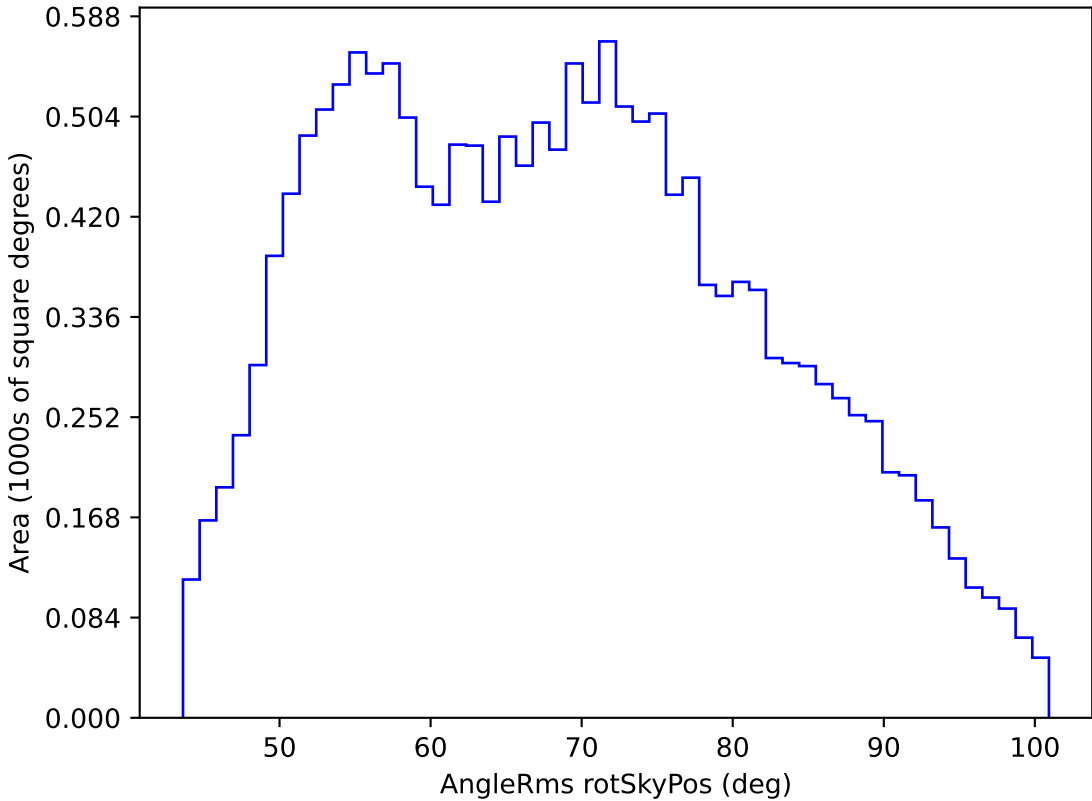
too_elab_r8_d3_gz_v3.4_10yrs WFD g band: AngleRms rotSkyPos
