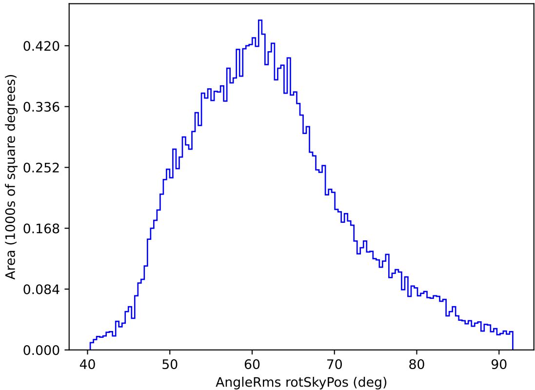
too_elab_r8_d3_gz_v3.4_10yrs All sky y band: AngleRms rotSkyPos
