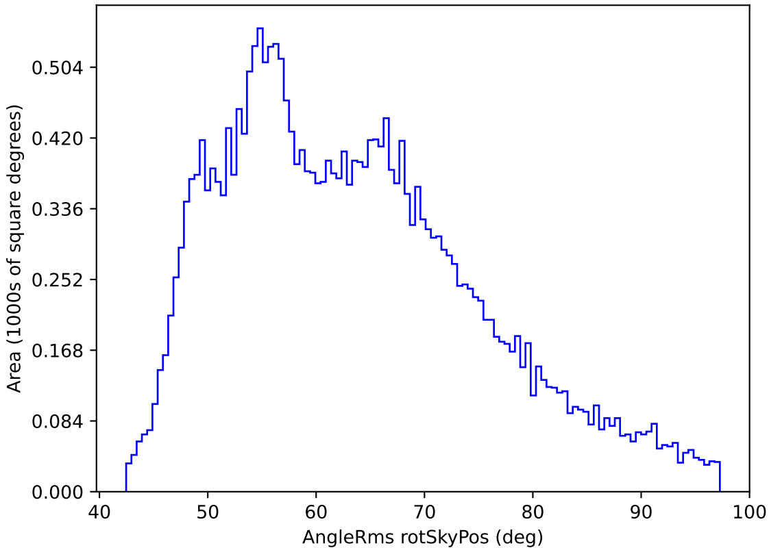
too_elab_r8_d3_gz_v3.4_10yrs All sky r band: AngleRms rotSkyPos
