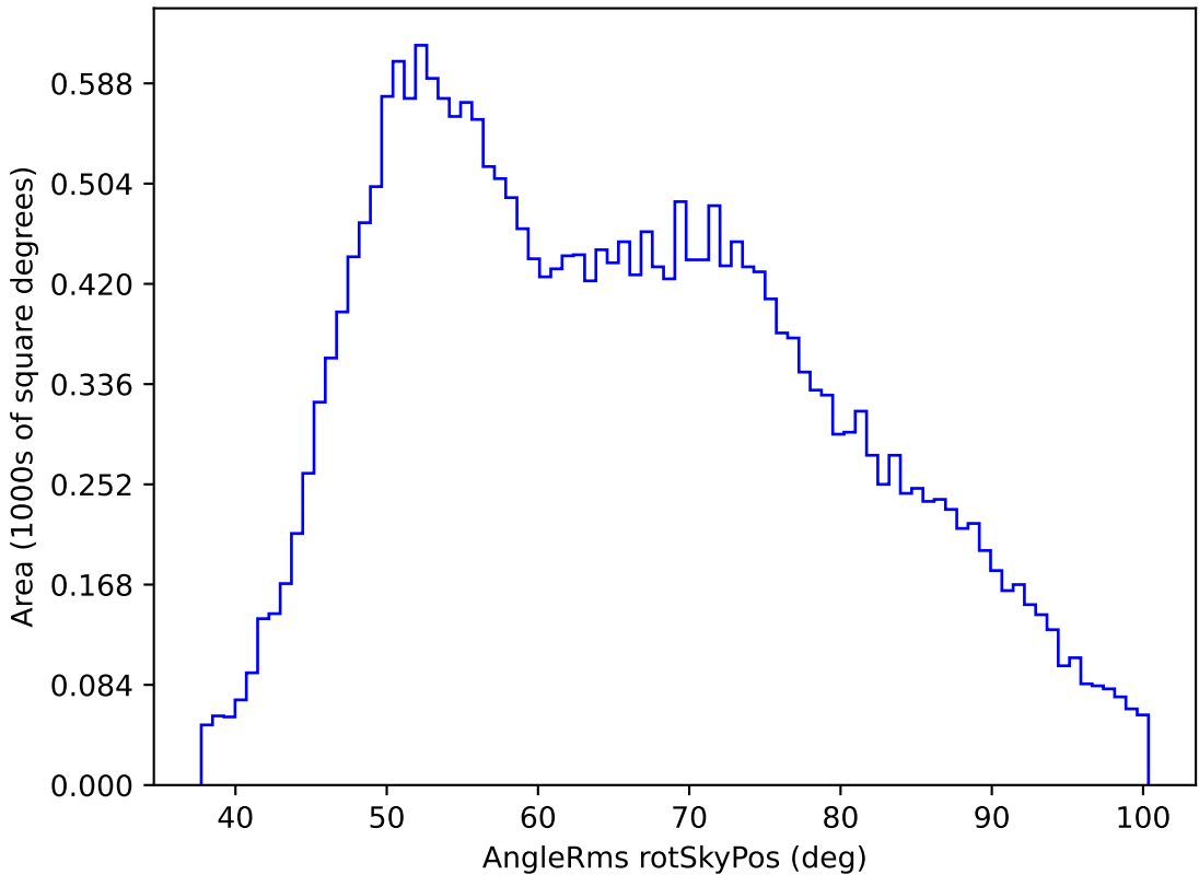
too_elab_r8_d3_gz_v3.4_10yrs All sky g band: AngleRms rotSkyPos
