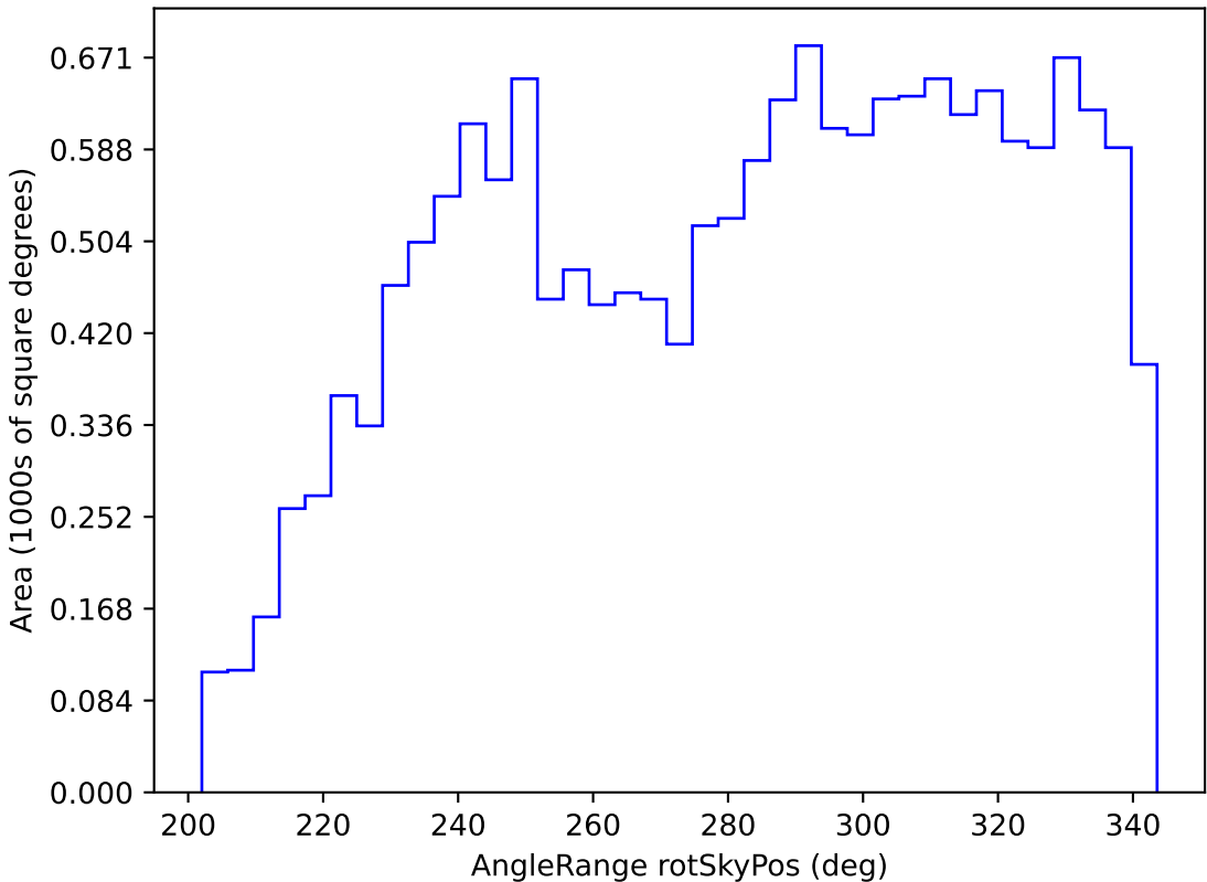
too_elab_r8_d3_gz_v3.4_10yrs WFD r band: AngleRange rotSkyPos
