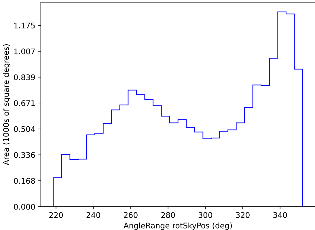
too_elab_r8_d3_gz_v3.4_10yrs WFD all bands: AngleRange rotSkyPos
