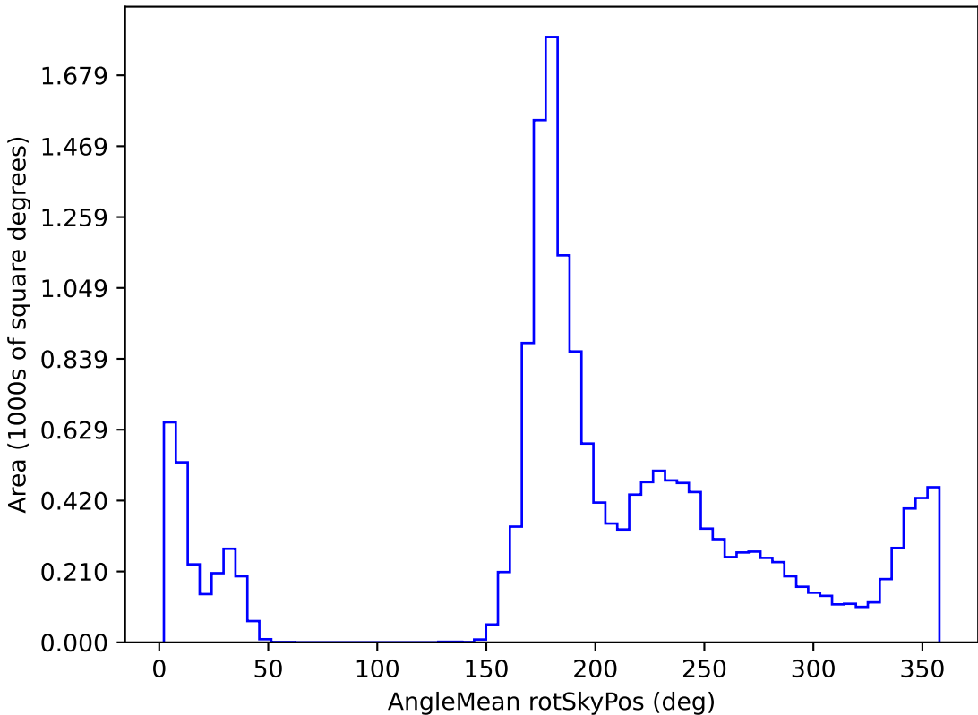
too_elab_r8_d3_gz_v3.4_10yrs WFD r band: AngleMean rotSkyPos
