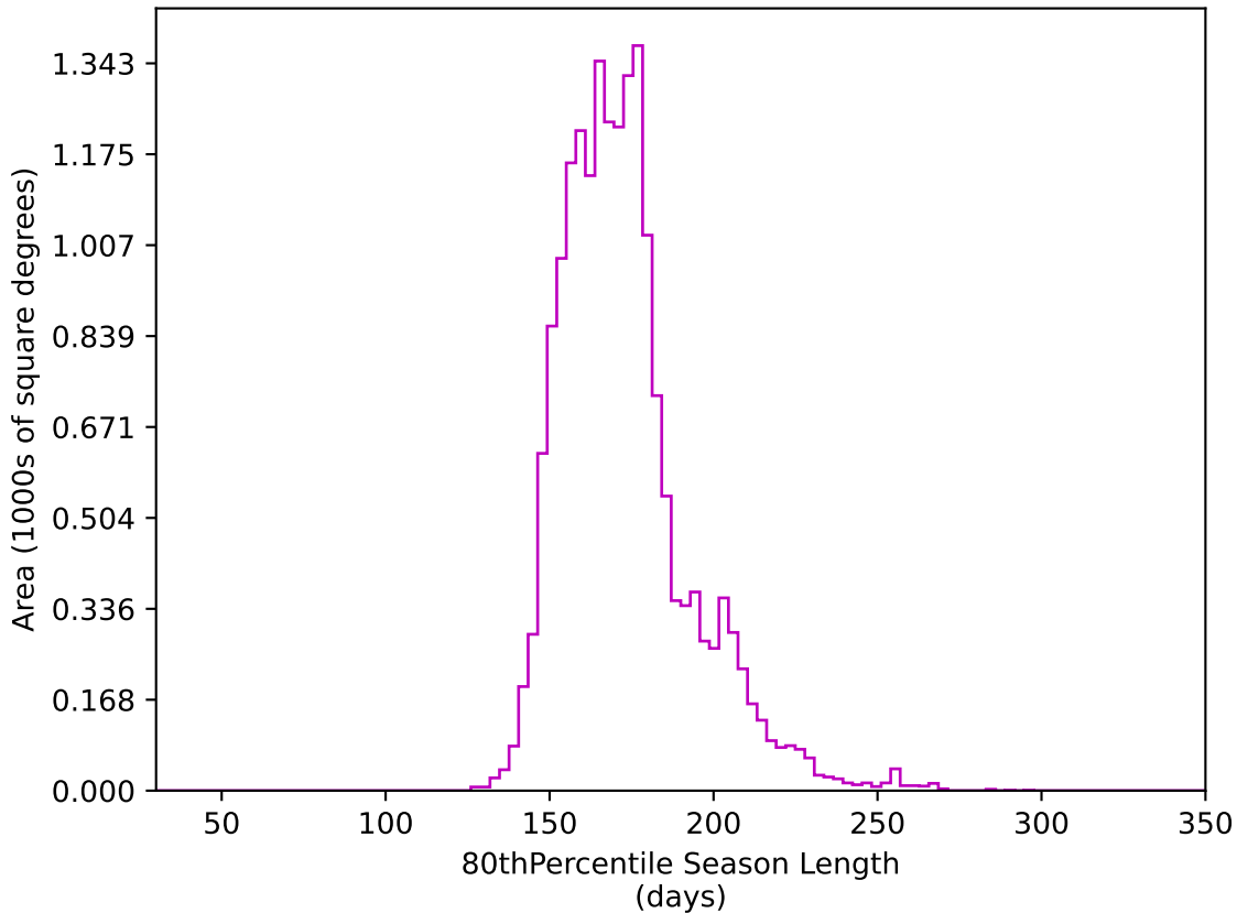
too_elab_r8_d3_gz_v3.4_10yrs WFD z band: 80thPercentile Season Length
