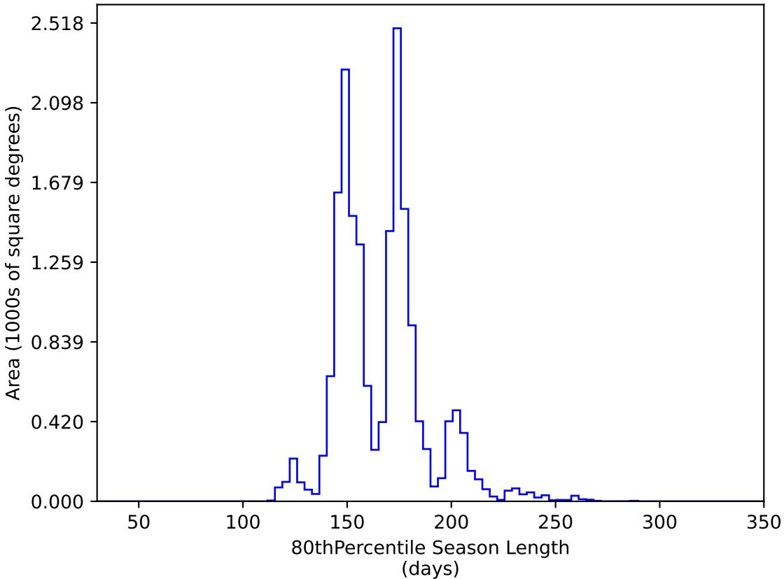
too_elab_r8_d3_gz_v3.4_10yrs WFD y band: 80thPercentile Season Length
