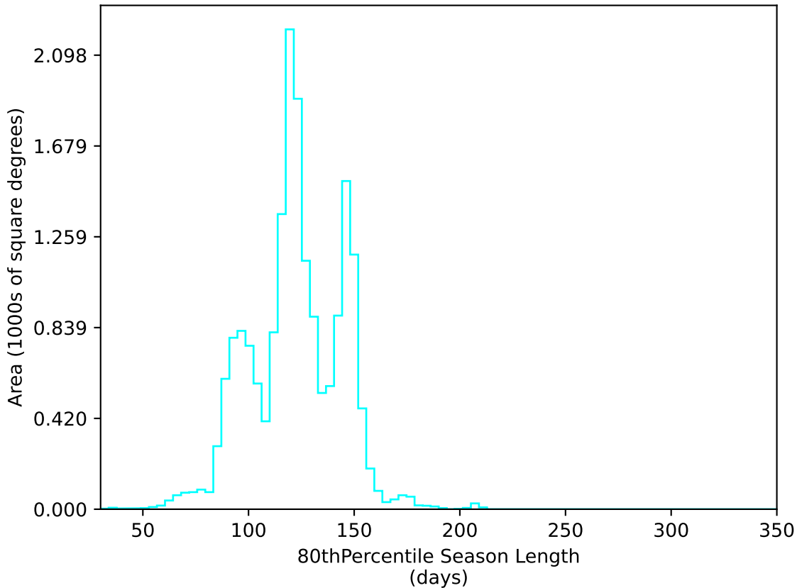
too_elab_r8_d3_gz_v3.4_10yrs WFD u band: 80thPercentile Season Length
